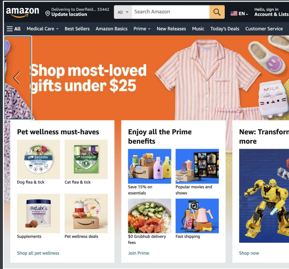
Shopping Prediction
