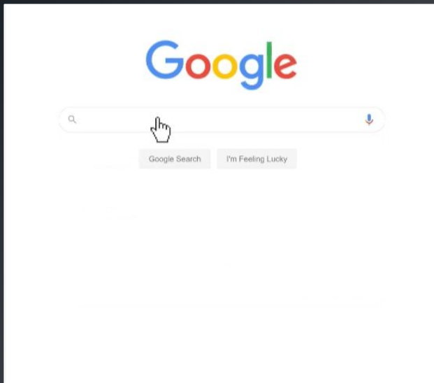
Google Search
