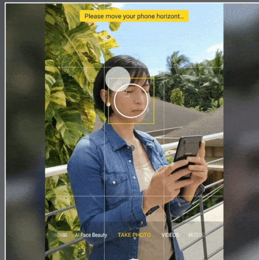
Smartphone Cameras
