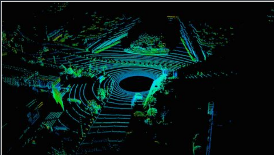
Self-Driving Cars
